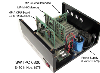
SWTPC6800 (1975)
