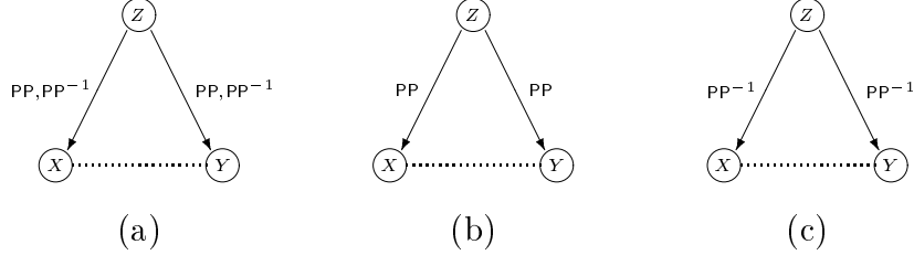
Fig. 3. Property 2: (a) is the original configuration, (b) and (c) are the only possible refinements of the relations to base relations.
