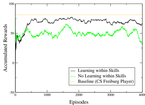
Fig. 1. Learner versus static goalkeeper with and without learning within skills
