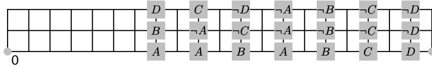
Fig. 1. GRID instance corresponding to (A \vee B \vee D) \wedge (A \vee \neg A \vee C) \wedge (B \vee \neg C \vee \neg D) . Locations with doors are marked with squares. The bottom left location contains the mobile and one key for each literal, opening the corresponding doors. The bottom right location contains an additional key. All keys must be moved to the bottom left location.
